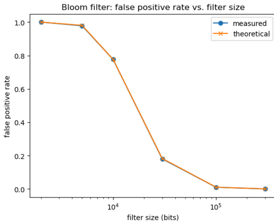
Figure 3: Graph of the empirical and theoretical false-positive rates for Bloom filter
